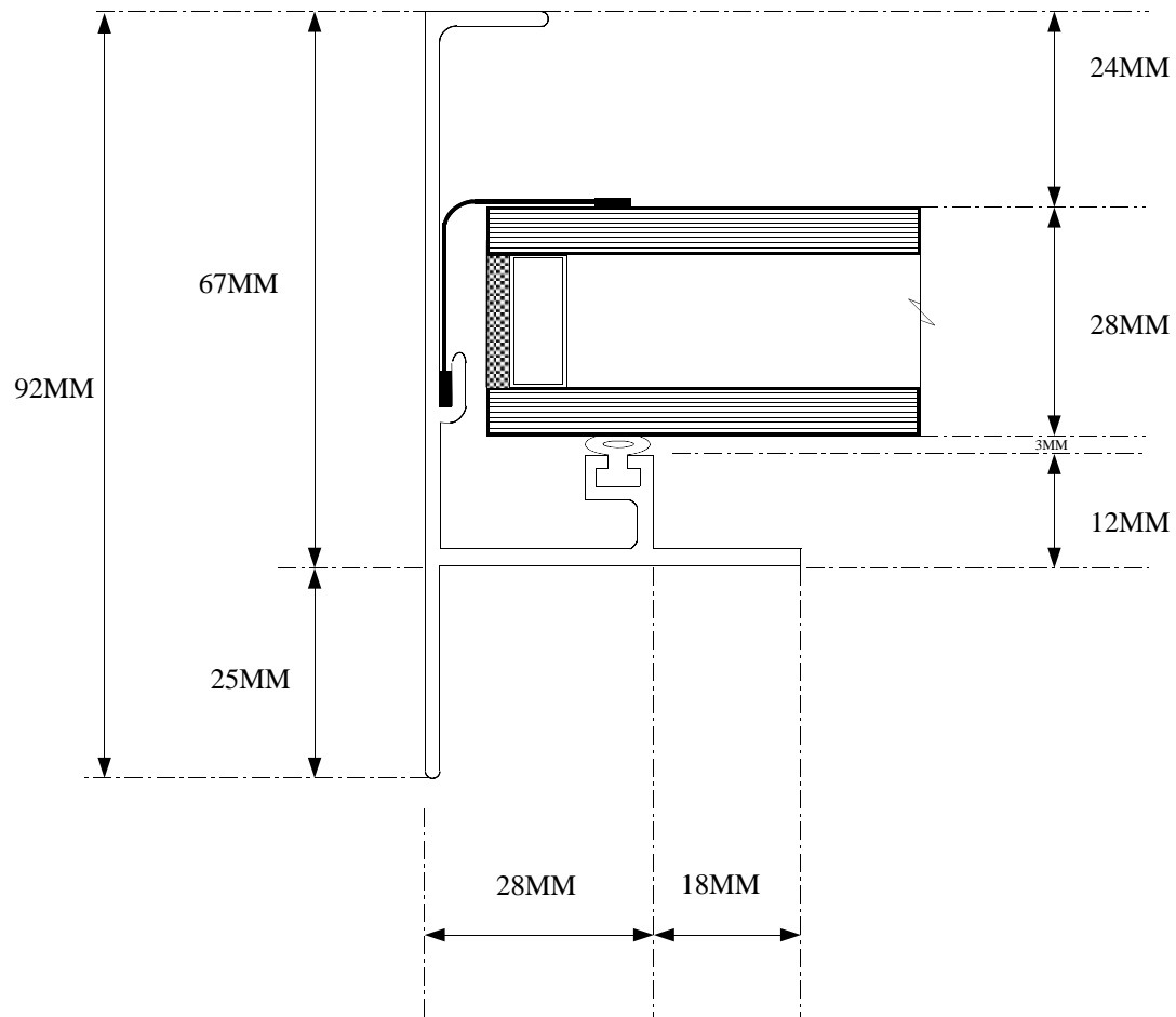
LWB64 LEAD WING FULL SIZE
