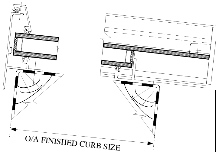
SECTION DOWN SLOPE OF DEADLIGHT
