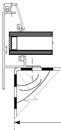
SECTION ACROSS DEADLIGHT NOT FULL SIZE
