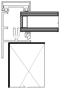
SECTION ACROSS DEADLIGHT NOT FULL SIZE
