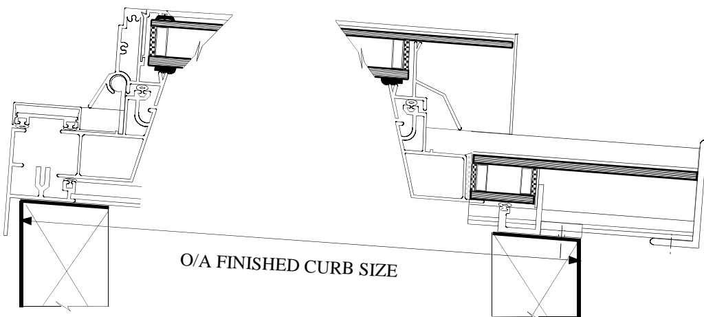
SECTION DOWN SLOPE NOT FULL SIZE
