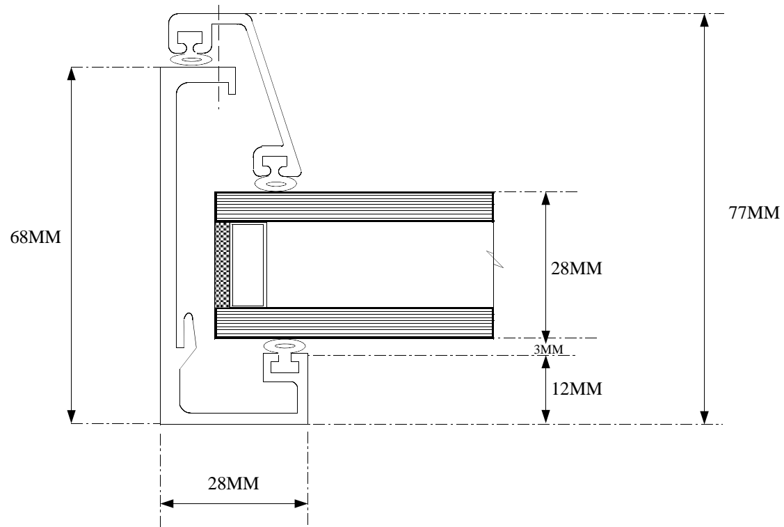
END BAR CEB 64 FULL SIZE
