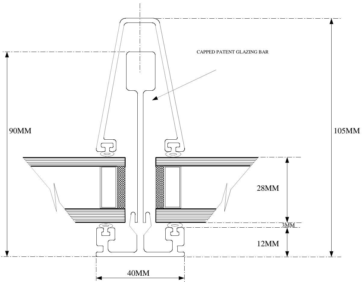
CB90 FULL SIZE
