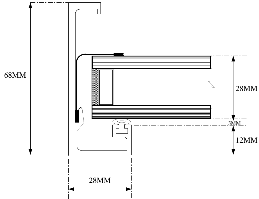
END BAR LWEB 64 FULL SIZE LEAD WING
