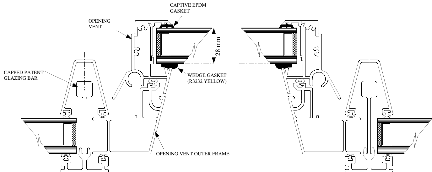
SECTION THROUGH GLAZING BARS & OPENING VENT
